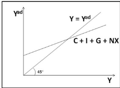
Keynesian Cross
