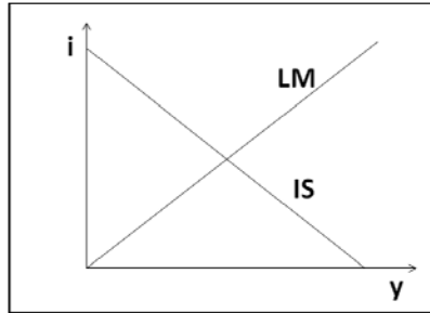
IS/LM model
