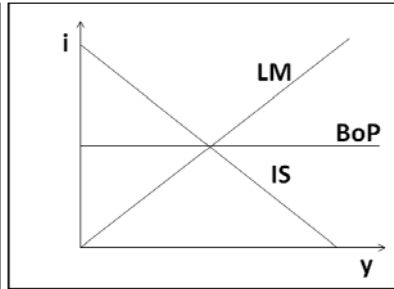
Mundell-Fleming
